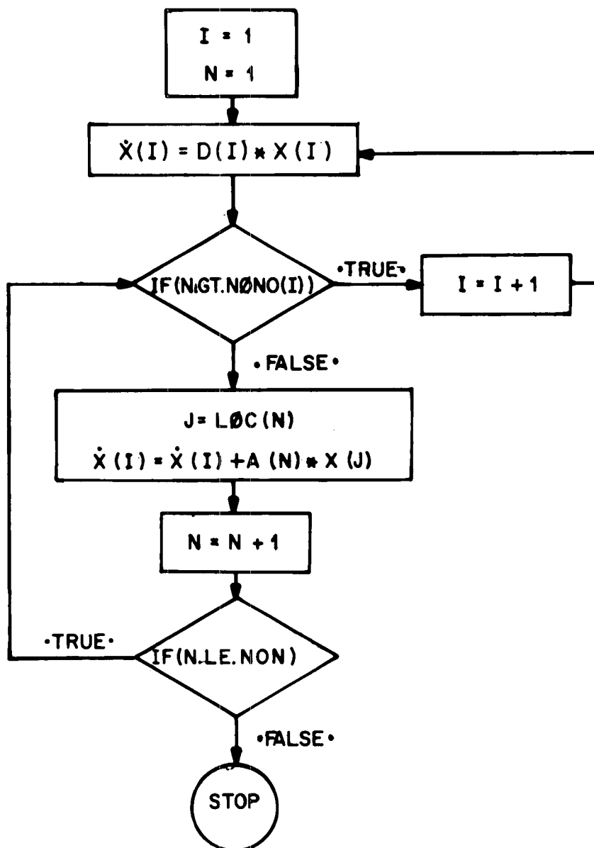
Fig. 2.1. Flowchart Illustrating Computational Algorithm Executed to Perform the Matrix Calculation \tilde{X} = A \tilde{X} .
